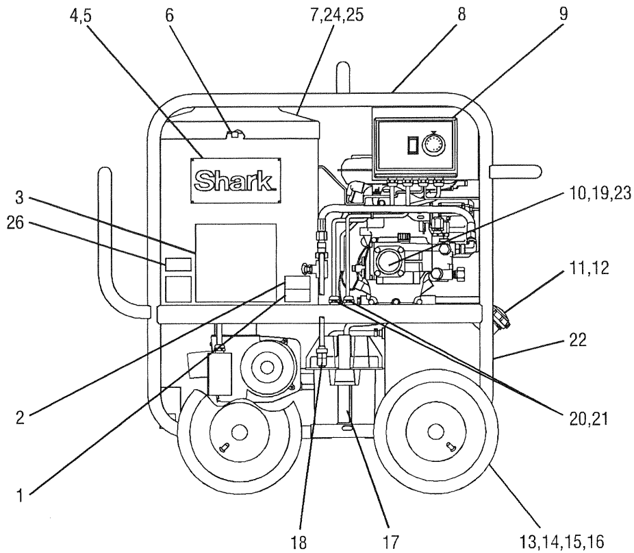
Figure 11 - Machine Assembly, Left View
